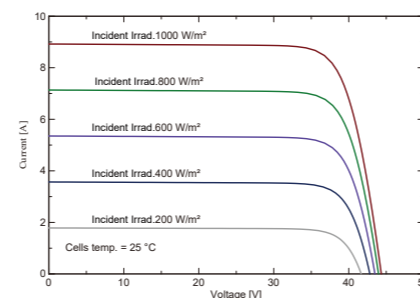
I-V Curve (SRP-280-BPB)
